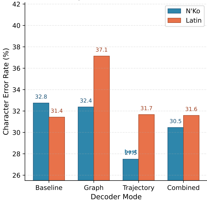
(A) CER by Script and Mode 297,053 pairs (237K train / 29K test)
