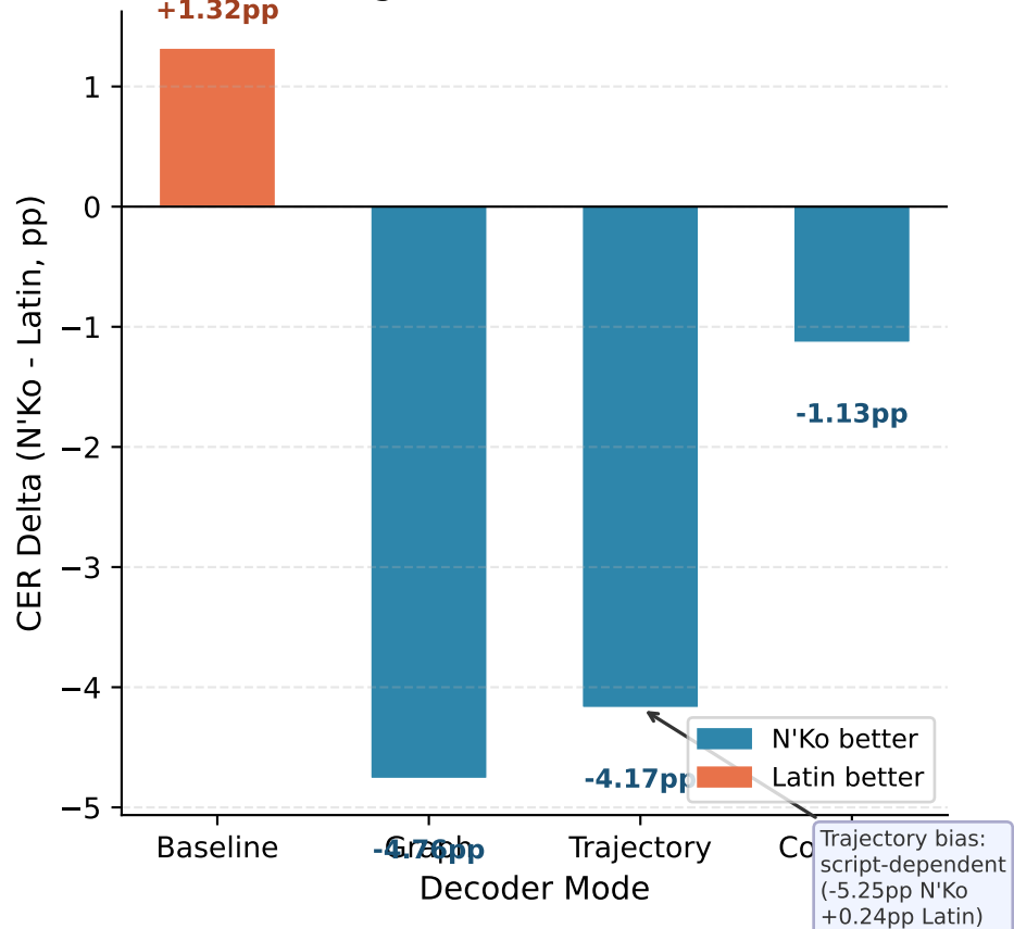
(B) Architecture Asymmetry (negative = N'Ko better)
